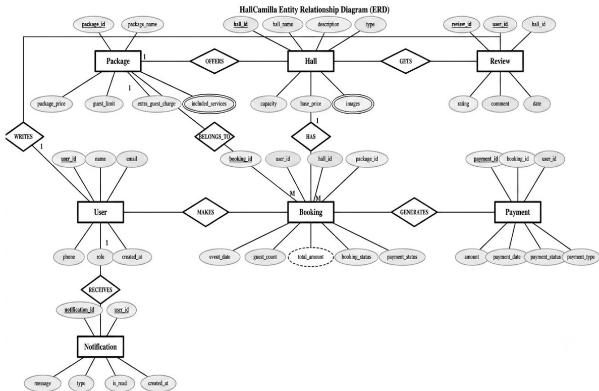
Figure 3. 31 : Entity Relationship Diagram
